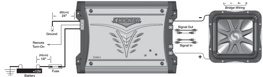
Bridged Operation (Mono) Minimum impedance of 4 ohms while in bridged operation
